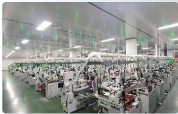
芯取 Centering
